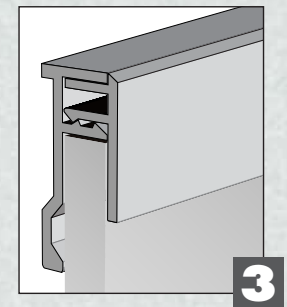
Clip-on fixing
